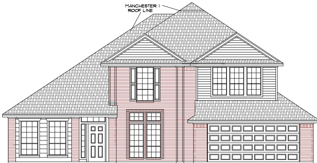
ELEVATION A (STANDARD)
