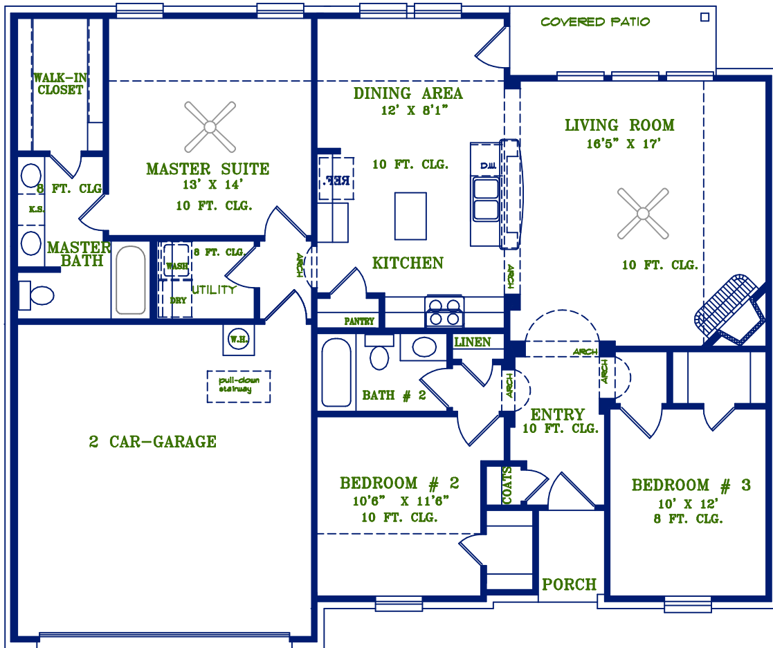
FLOOR PLAN
