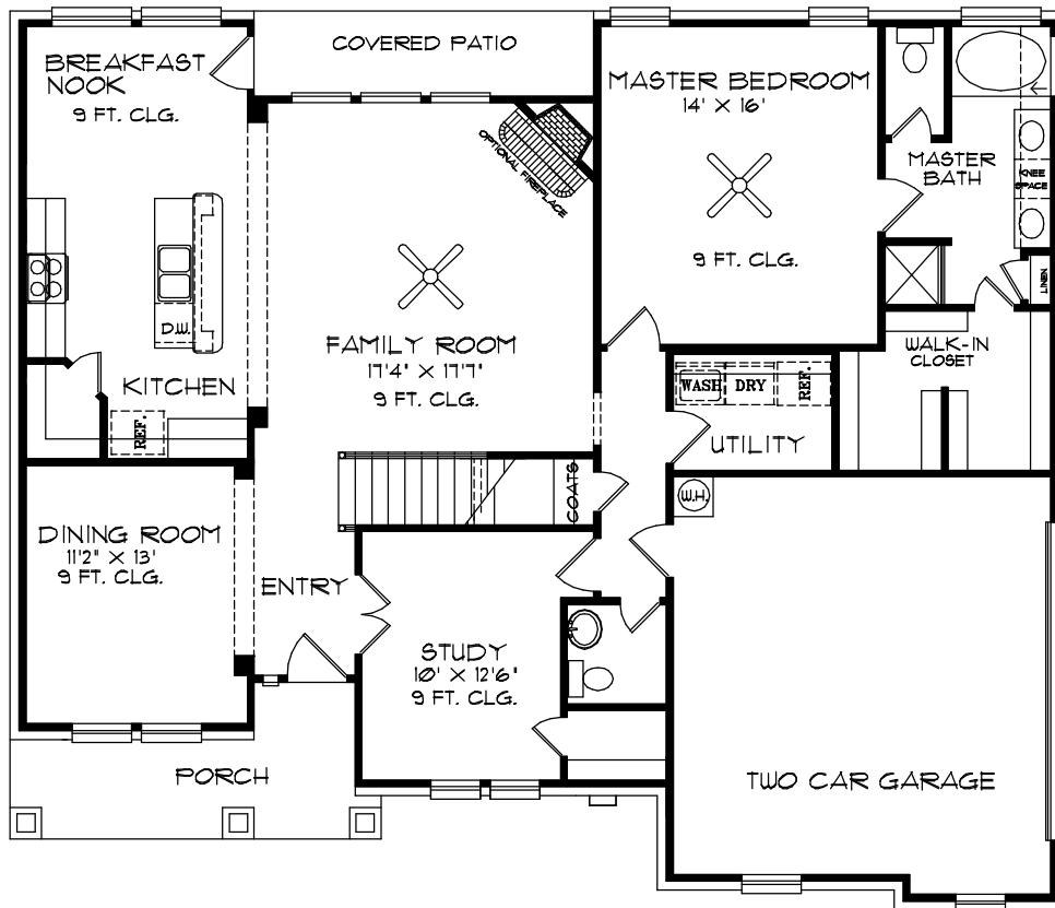
FIRST FLOOR PLAN 1640 SQ. FT. FIRST FLOOR LIVING AREA
